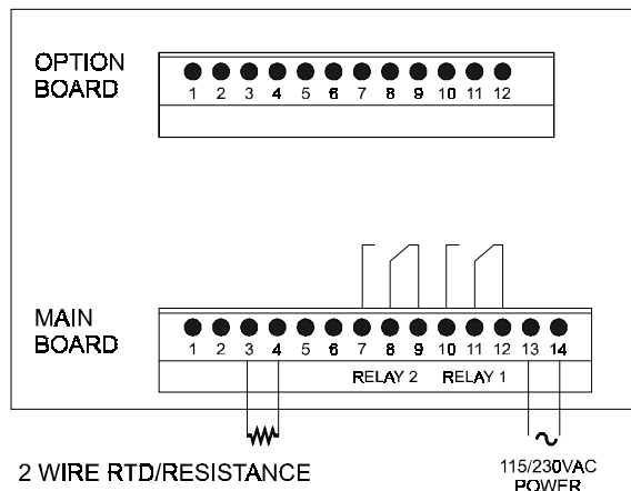
S2PM REAR VIEW WITH OPTION BOARD
